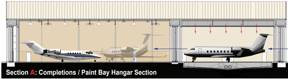
Paint Hangar Filter Bank
